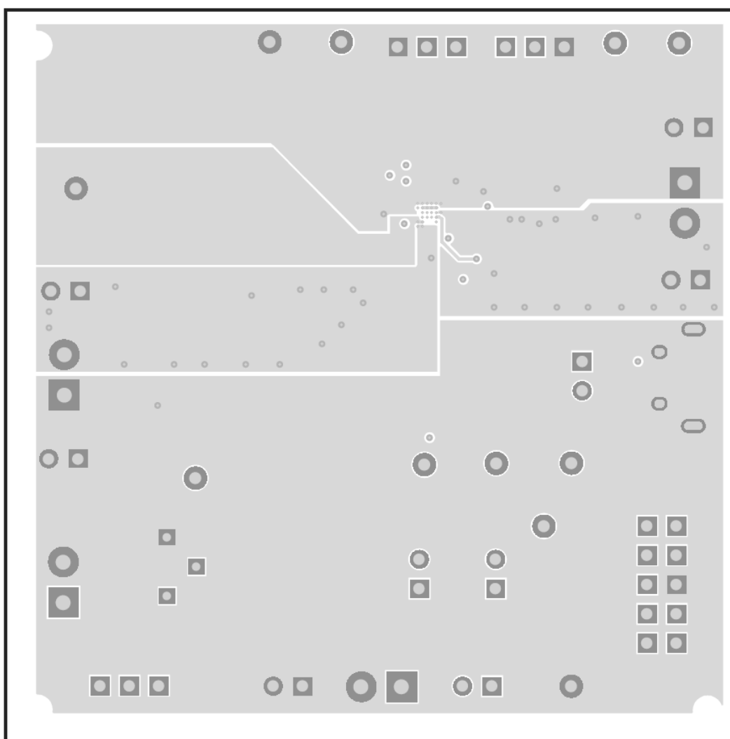
Figure 10. Bottom Layer
