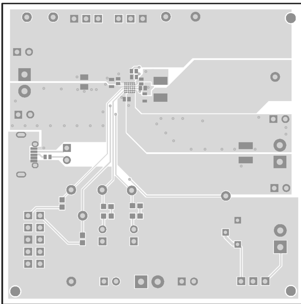
Figure 7. Top Layer
